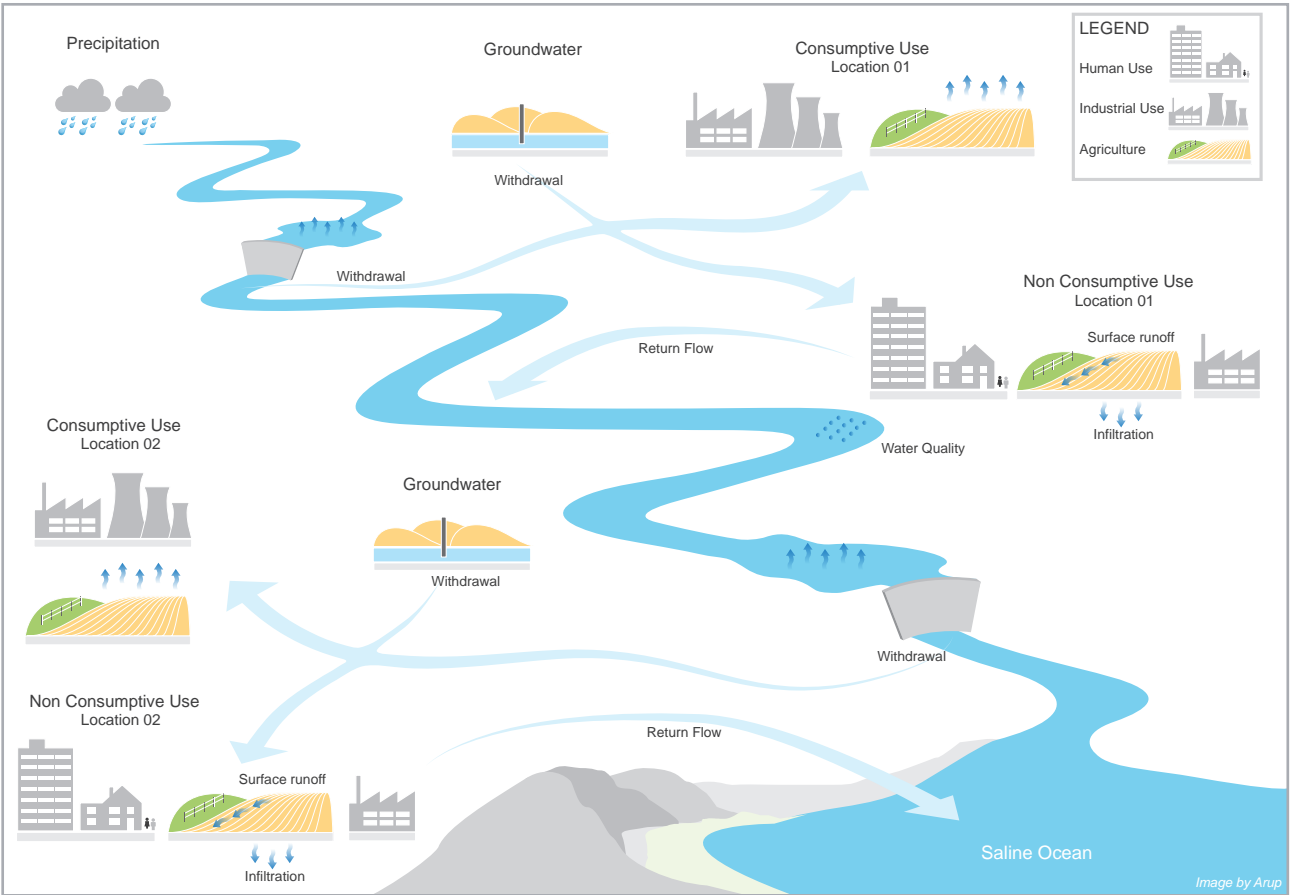
Semi-circularity of water flows within a basin
